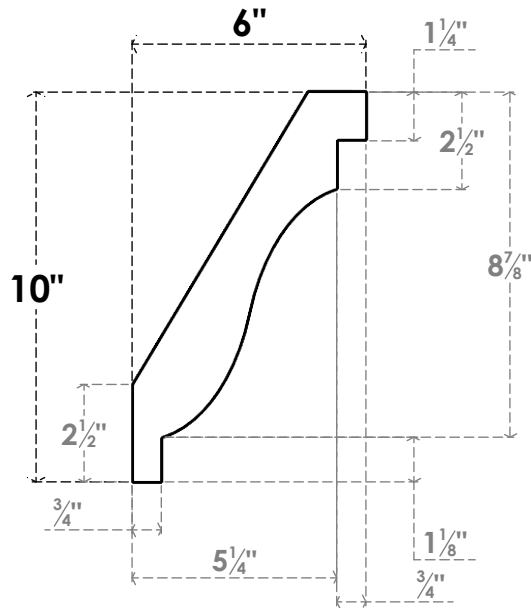
SIDE PROFILE
